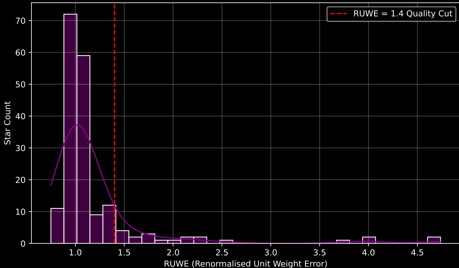
GAPOGEE DR17 Field [072+51_MGA] RUWE Distribution (n= 184)
