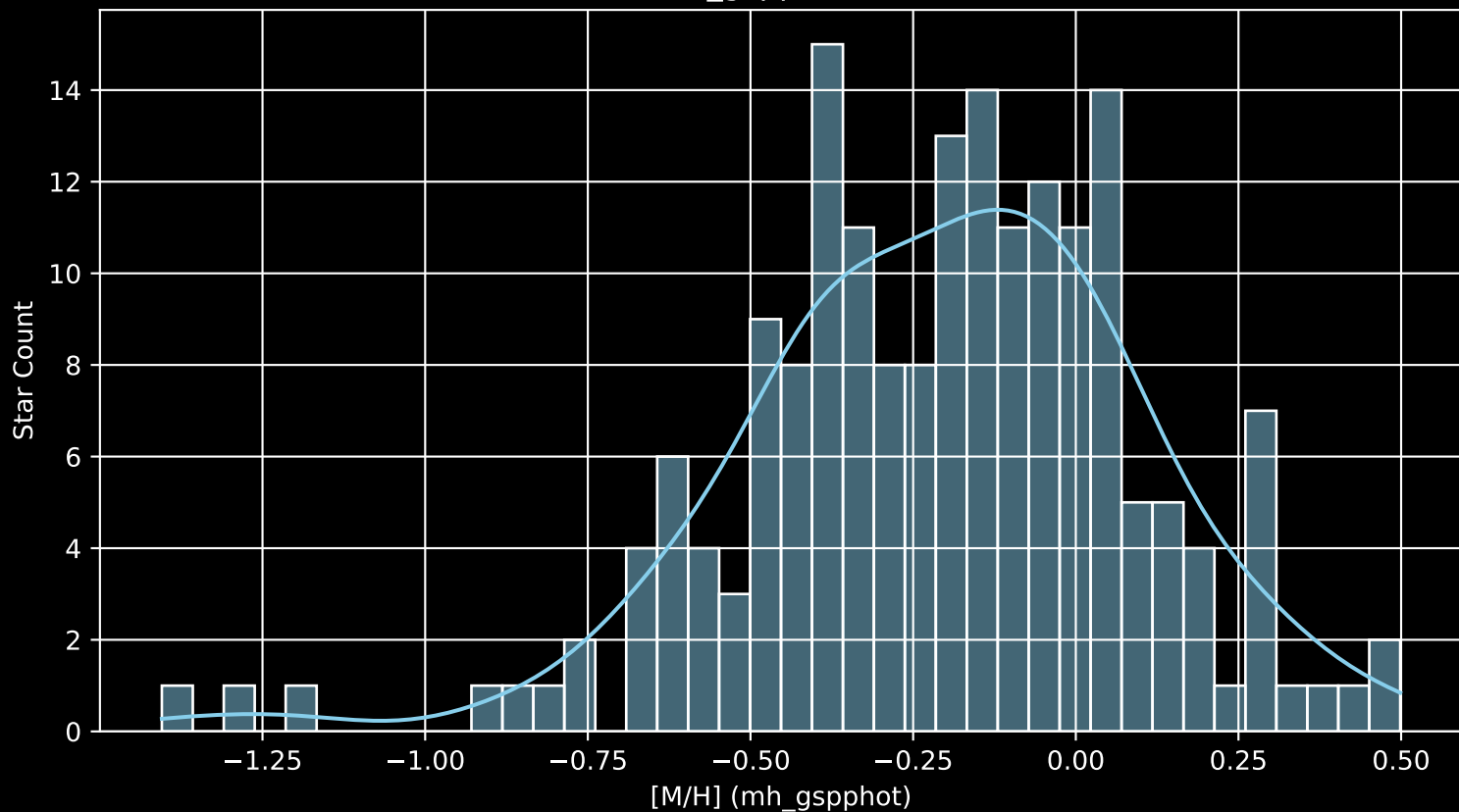
APOGEE DR17 Field: [072+51_MGA [M/H] (mh_gspphot) (n= 186)
