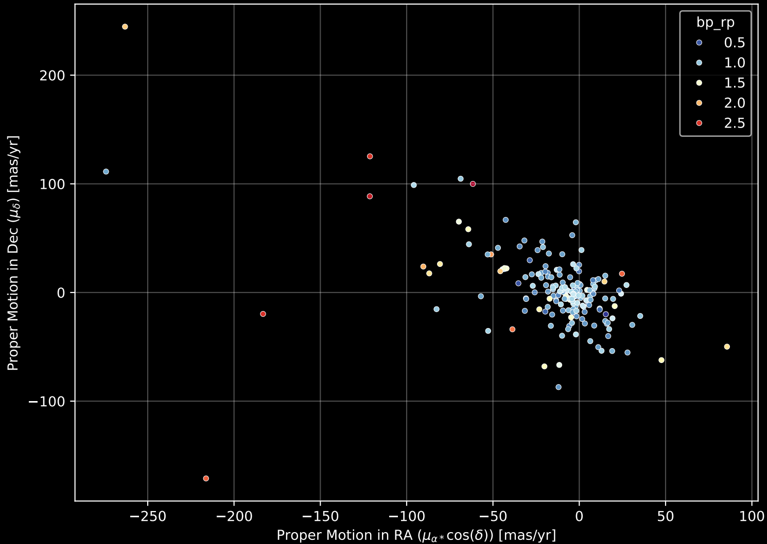
APOGEE DR17 Field: [072+51_MGA] Proper Motion Diagram (n= 188)
