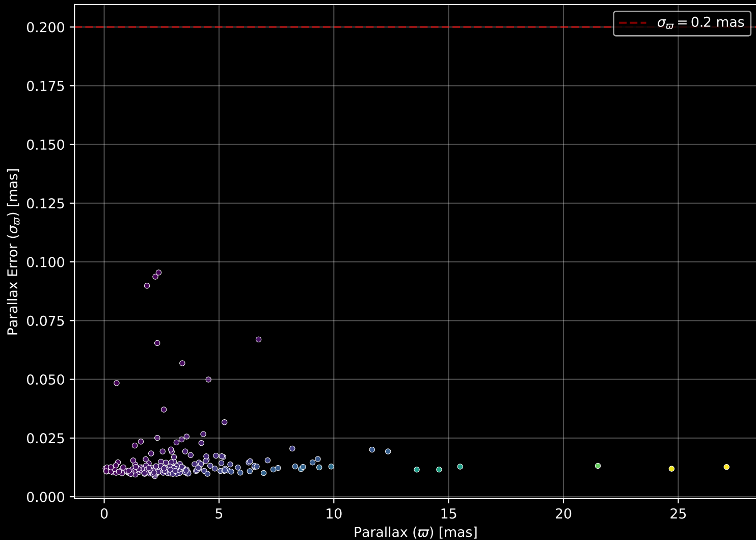
APOGEE DR17 Field: [072+51_MGA] Parallax Quality (n= 188)
