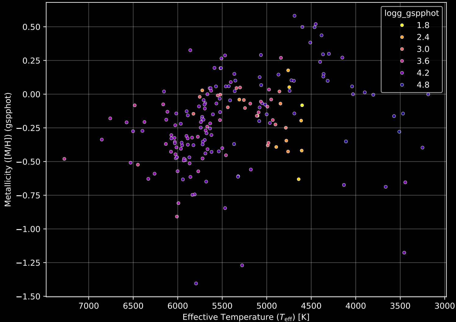
APOGEE DR17 Field: [072+51_MGA] Stellar Population Parameters (n= 188)
