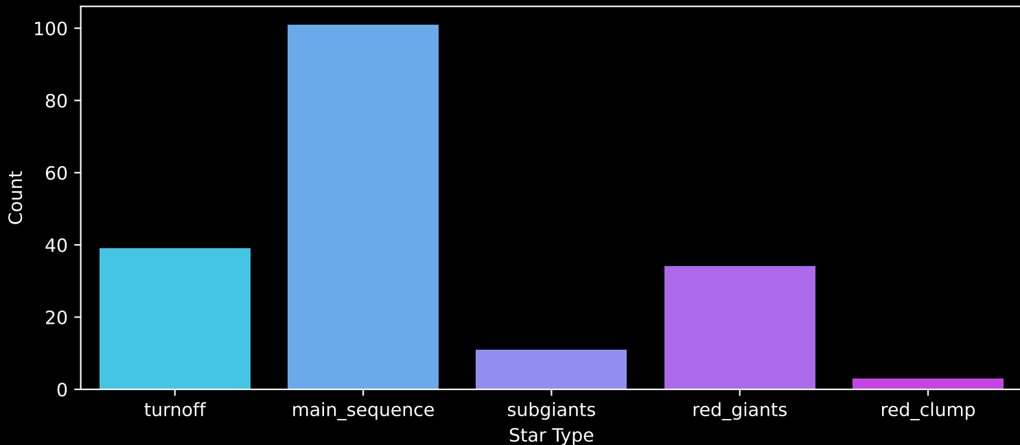
APOGEE DR17 Field: [072+51_MGA] Count plot of Star Type
