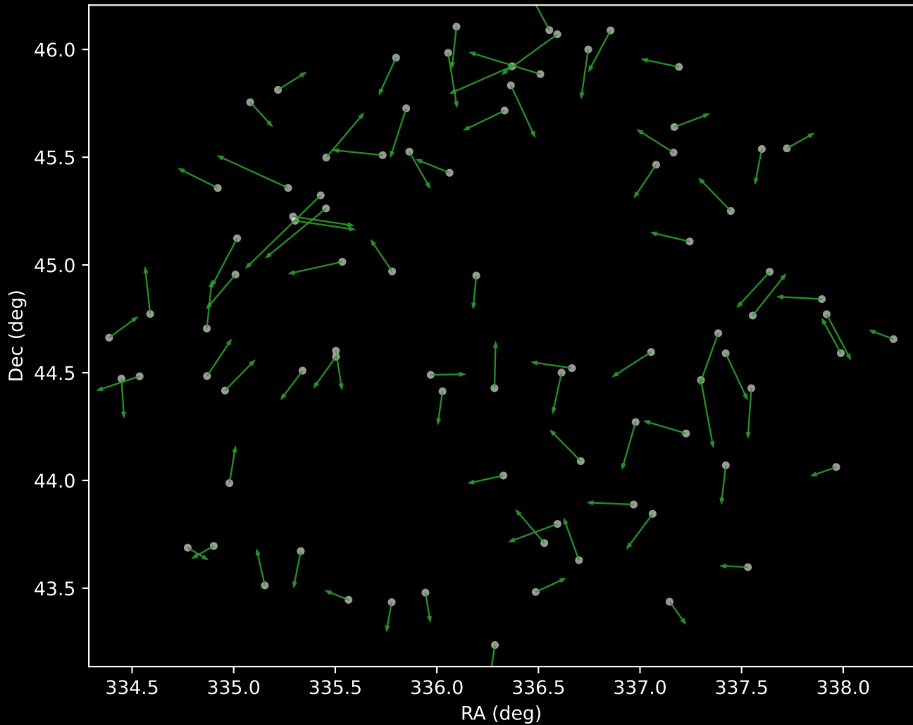
APOGEE DR17 Cluster 4 Proper Motion Vectors (n=86)
